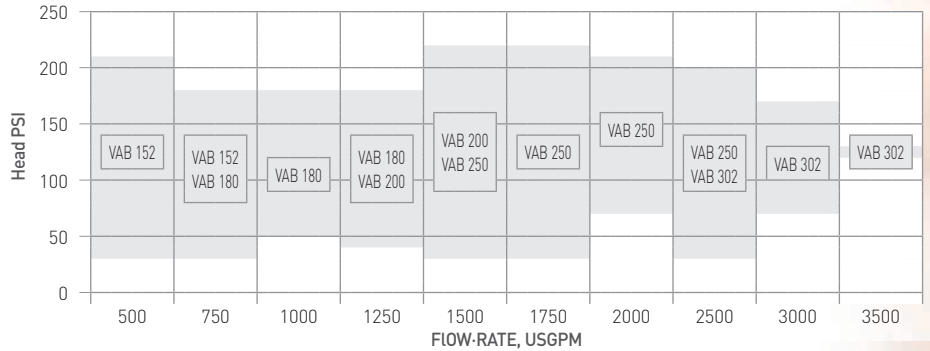
VERTICAL PUMPS AT 1n0 RPM, F. M. APPROVED RANGE HEAD. PSI FLOW-RATE USGPM
